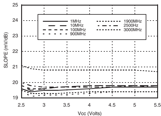
LOGOUT Slope vs. Supply Voltage, T_A = +25^\circ C
