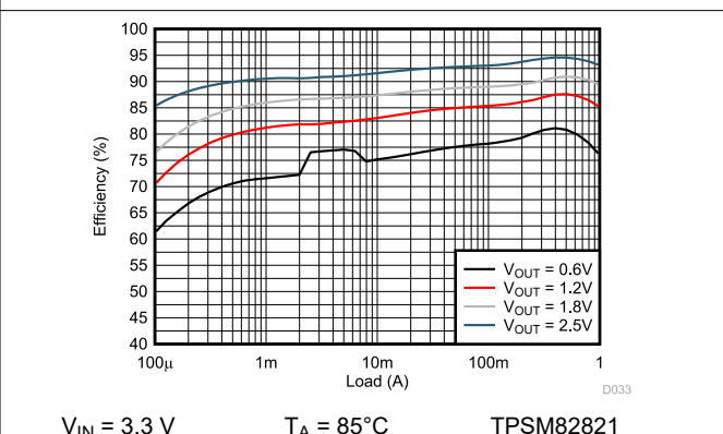
Figure 9-6. Efficiency
