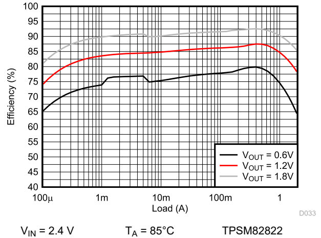
Figure 9-36. Efficiency
