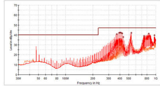
R_{LOAD} = 1 \Omega , V_{IN} = 5.5 \text{ V} (battery supply), V_{OUT} = 1.8 \text{ V} , tested on TPSM82822EVM-080
