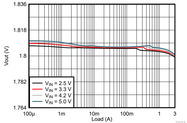
Figure 9-75. Load Regulation
