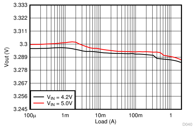
Figure 9-44. Load Regulation
