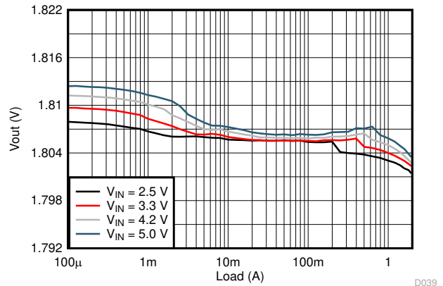
Figure 9-42. Load Regulation
