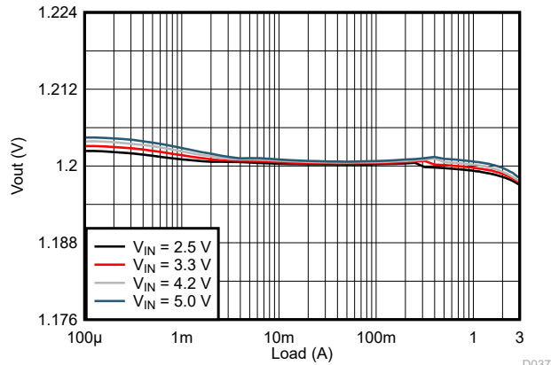
Figure 9-76. Load Regulation
