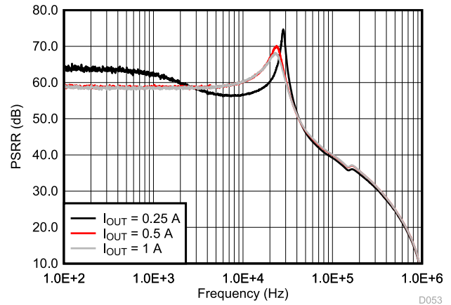
Figure 9-28. Power Supply Rejection Ratio (PSRR)
