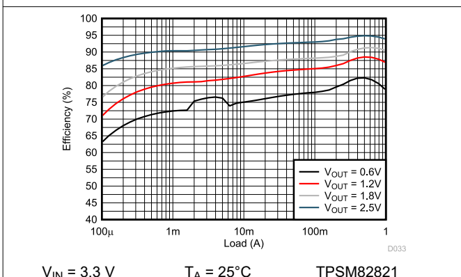
Figure 9-5. Efficiency
