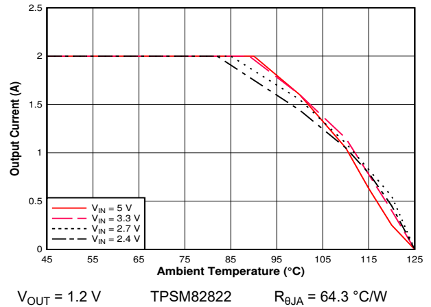
Figure 9-38. Safe Operating Area
