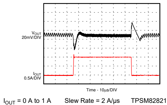
Figure 9-25. Load Transient
