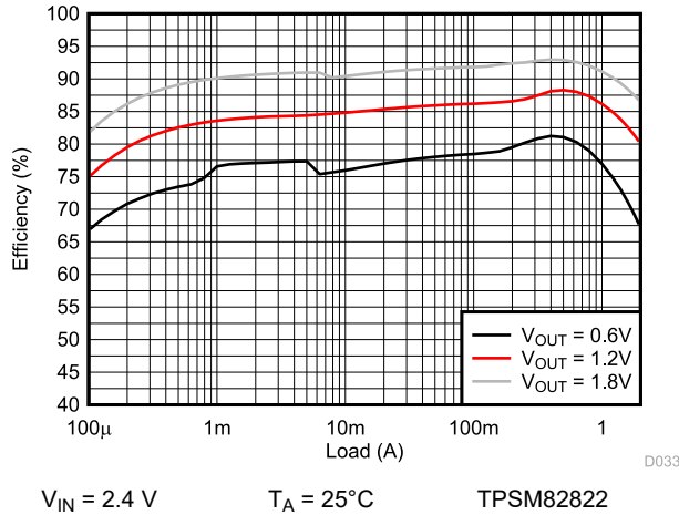
Figure 9-35. Efficiency
