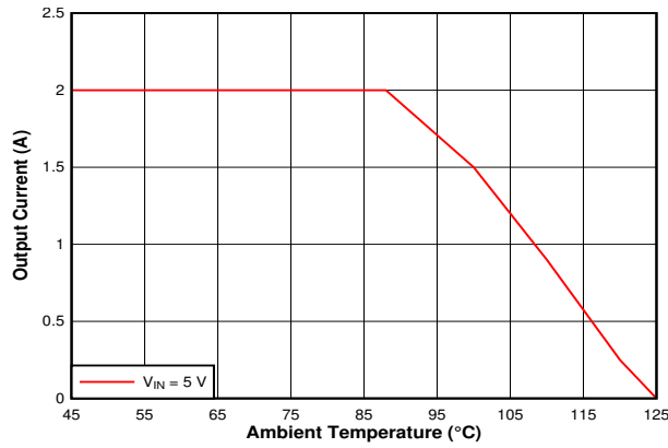
Figure 9-41. Safe Operating Area
