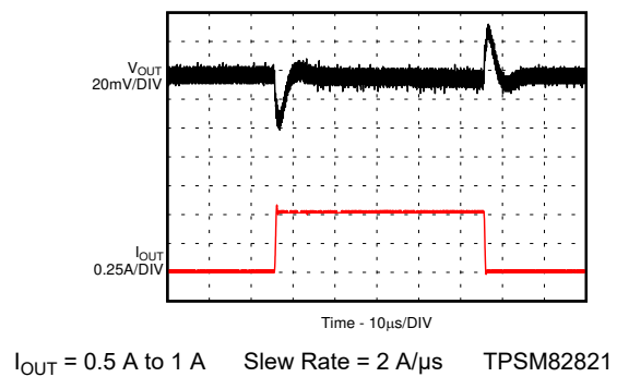
Figure 9-26. Load Transient
