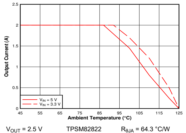
Figure 9-40. Safe Operating Area
