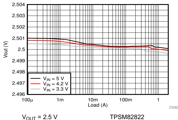
Figure 9-45. Load Regulation
