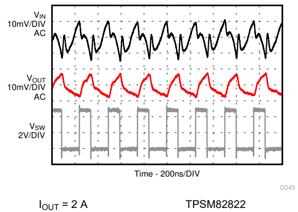
Figure 9-52. Input and Output Ripple in PWM Mode
