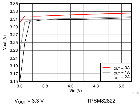
Figure 9-51. Line Regulation
