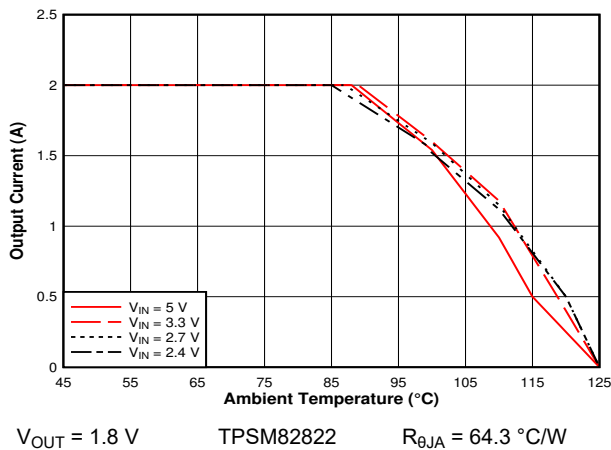
Figure 9-39. Safe Operating Area
