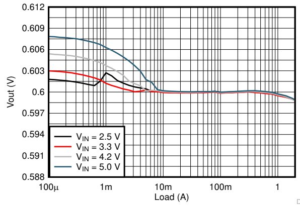
Figure 9-42. Load Regulation
