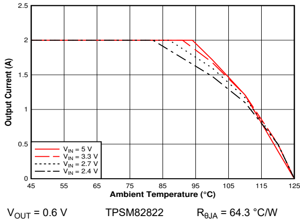
Figure 9-37. Safe Operating Area
