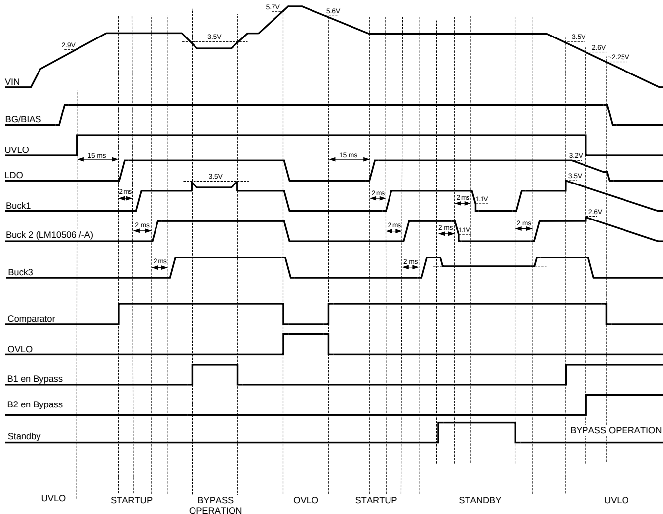
Figure 21. Operating Modes
