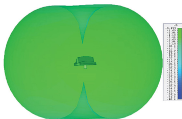
3D Gain Plot Side (700MHz)
