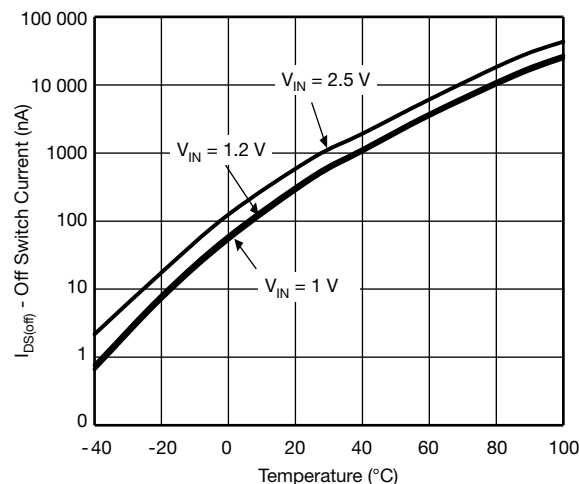
Fig. 11 - Off Switch Current vs. Temperature
