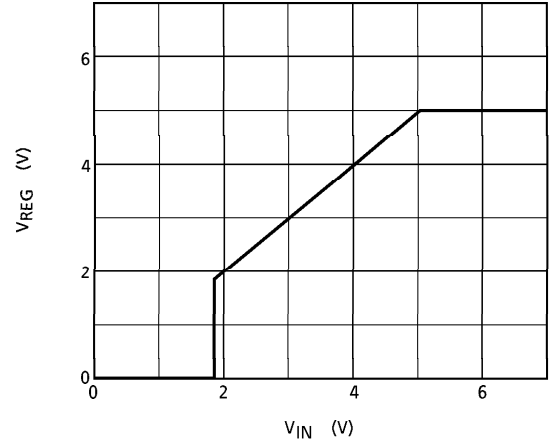
INPUT-OUTPUT CHARACTERISTICS
