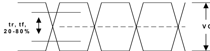
Figure 3. ECL/LVPECL Output
