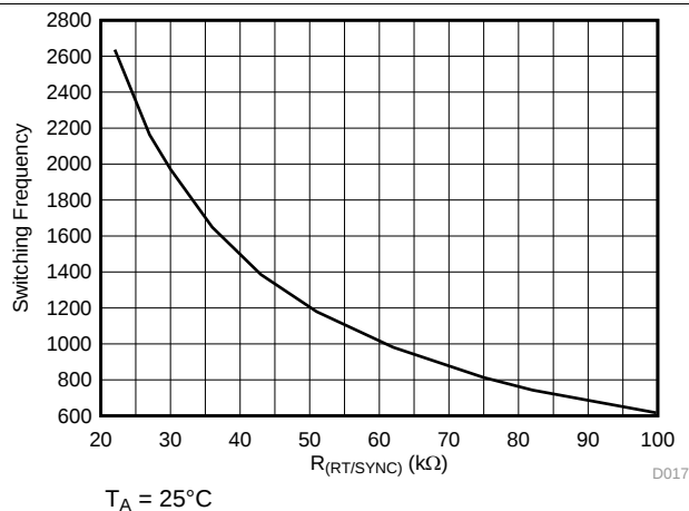
图 17. Switching Frequency vs R_{(RT/SYNC)} High Range
