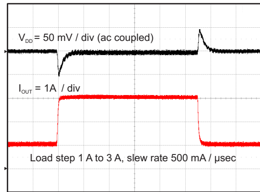
图 62. V_{DD} Output Transient Response
