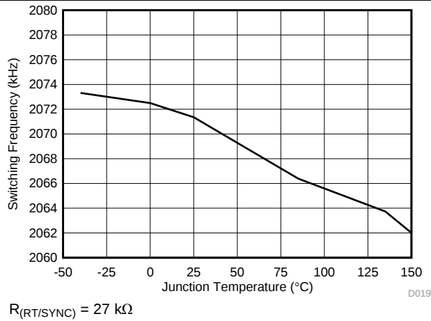
图 19. Switching Frequency vs Temperature
