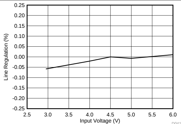
图 51. V_{DD} Output Line Regulation, I_{OUT} = 2 A
