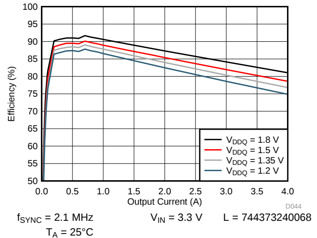
图 36. Efficiency
