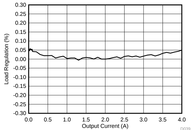
图 50. V_{DD} Output Load Regulation, V_{IN} = 5 V
