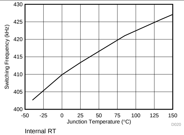
图 20. Switching Frequency vs Temperature
