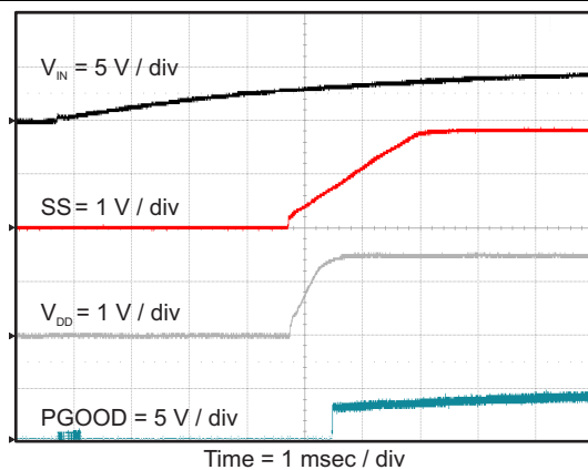
图 55. V_{DD} Start-Up Relative to V_{IN}
