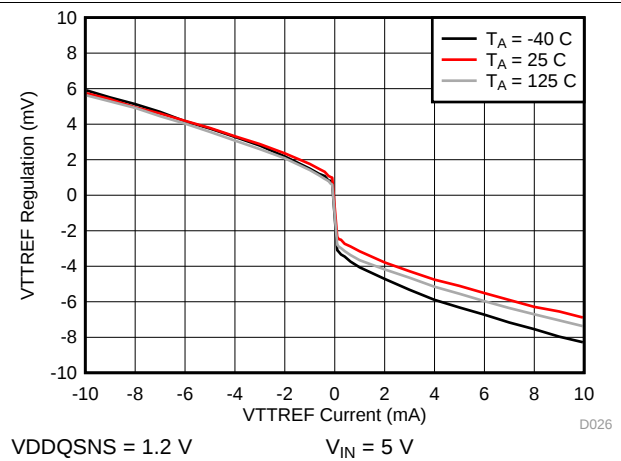
图 28. VTTREF Regulation to VDDQSNS/2 vs I VTTREF
