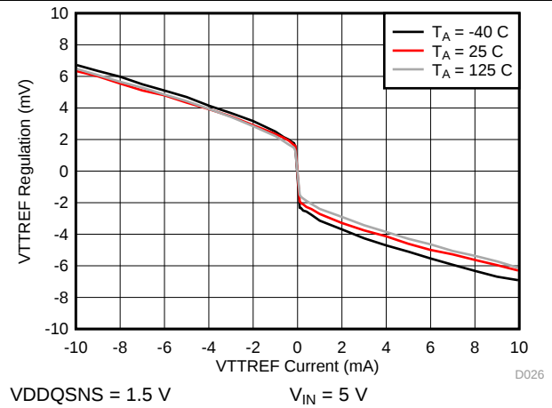
图 26. VTTREF Regulation to VDDQSNS/2 vs I VTTREF
