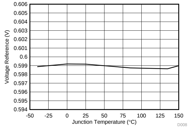
图 8. Voltage Reference vs Temperature
