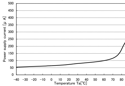
I_{OCT} timer mode(sub oscillation) temperature characteristics Vcc:5.5V, LVD is Off
