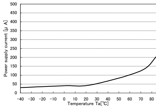
I_{OCH} stop mode (sub oscillation) temperature characteristics Vcc:5.5V, LVD is Off
