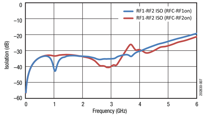
Figure 7. Isolation vs Frequency
