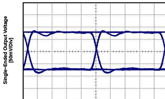
ELECTRICAL EYE-DIAGRAM AT 2.125 Gbps WITH K28.5 PATTERN
