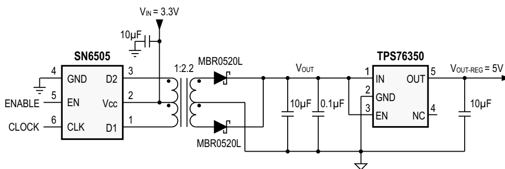
Figure 42. Typical Application Schematic
