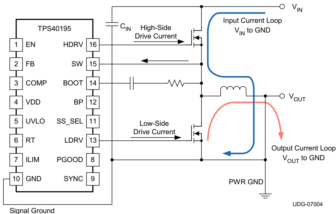
Figure 22. Layout Suggestion
