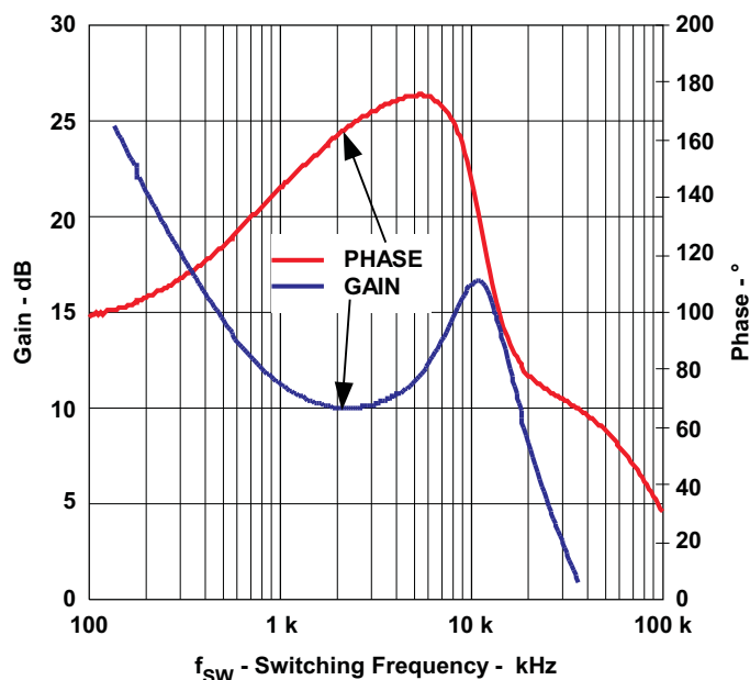
Figure 28. Final Bode Plot
