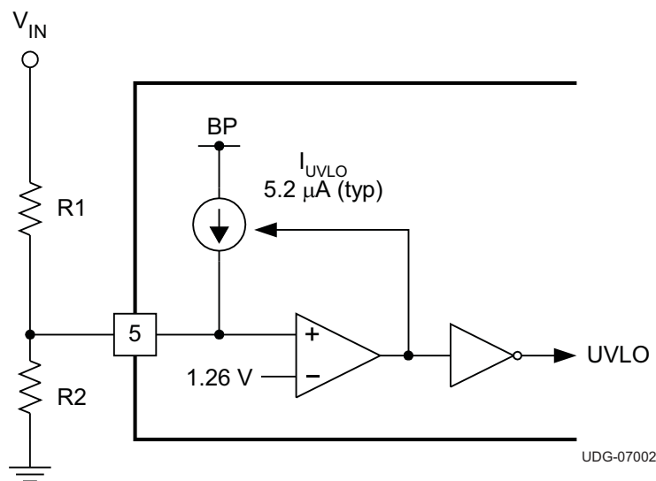
Figure 20. Undervoltage Lockout
