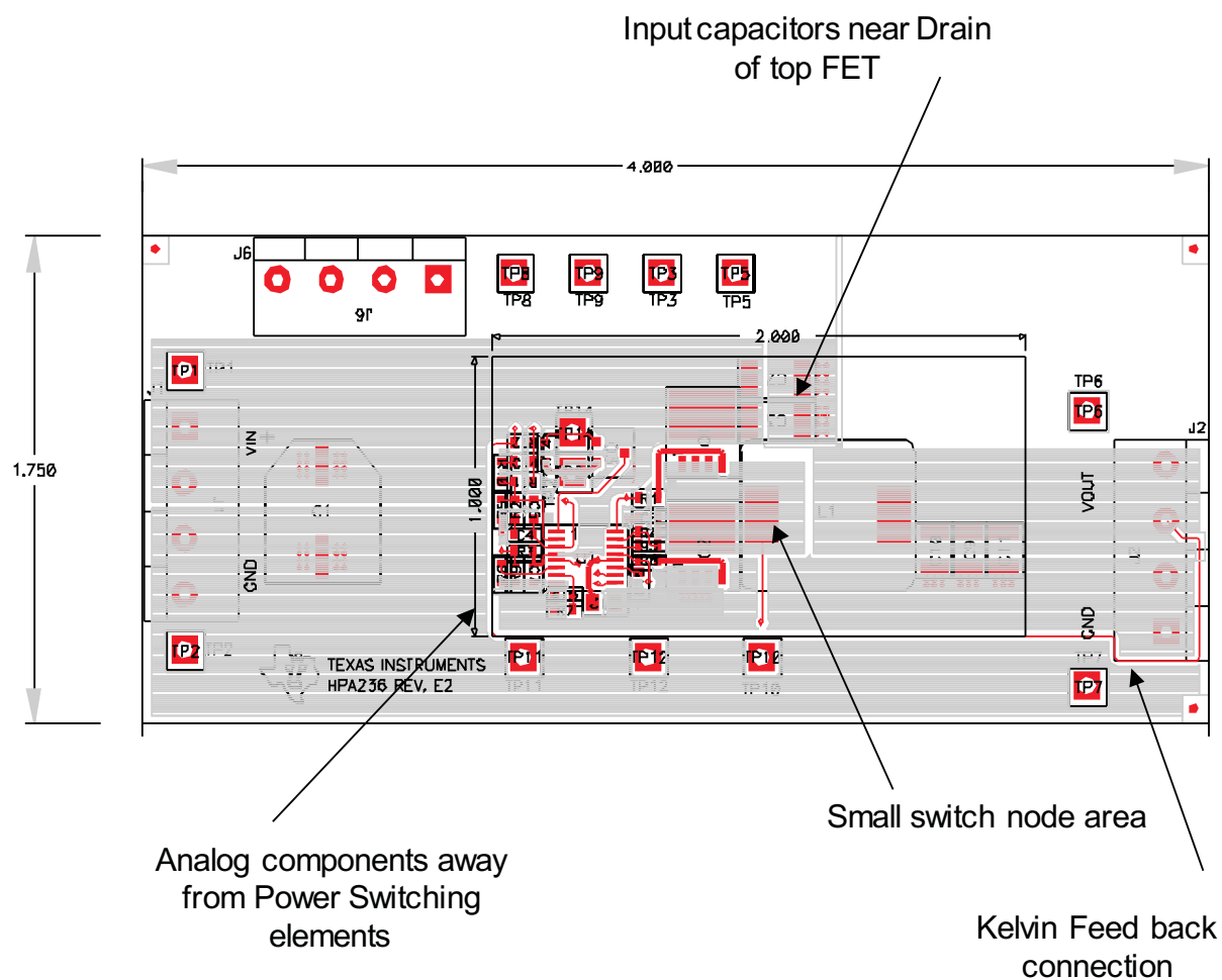
Figure 23. Board Layout
