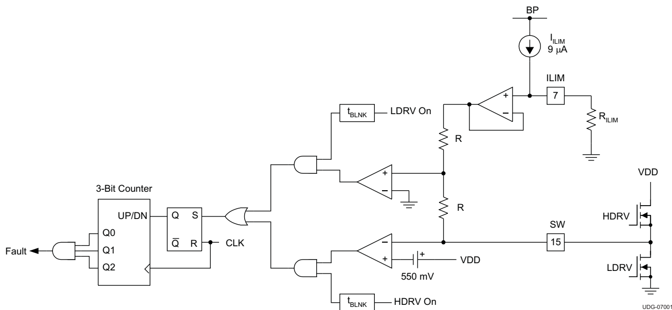
Figure 21. Overcurrent
