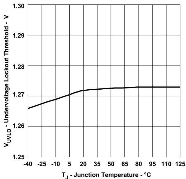
UNDERVOLTAGE LOCKOUT THRESHOLD vs JUNCTION TEMPERATURE
