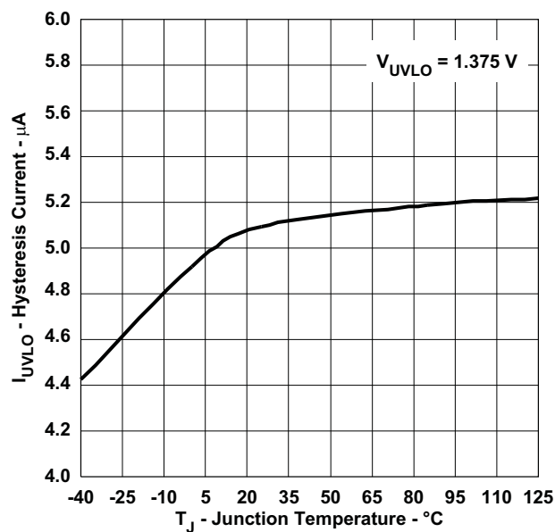
UNDERVOLTAGE LOCKOUT HYSTERESIS vs JUNCTION TEMPERATURE
