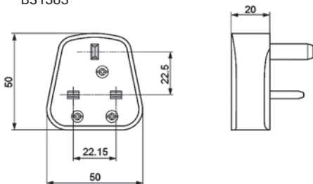
BS1363
