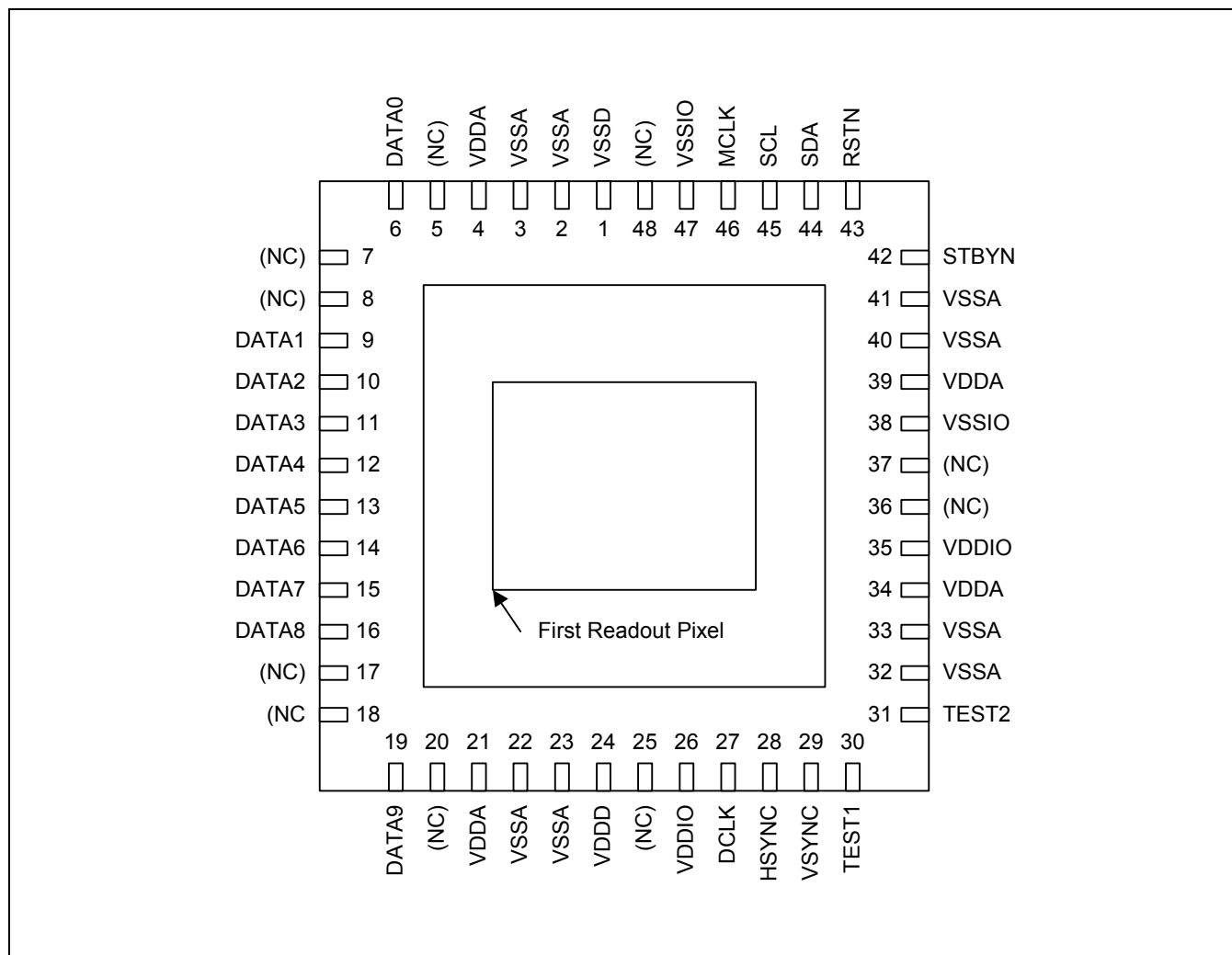
Figure 3. Pin Configuration
