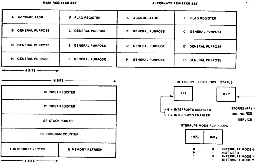
Fig. 4. CPU Registers
