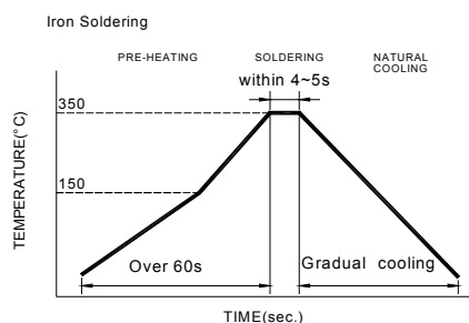
Iron Soldering times : 1 times max Fig.2
