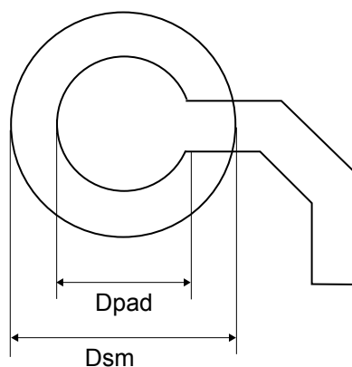
Figure 92. WLCSP132 - Recommended footprint
