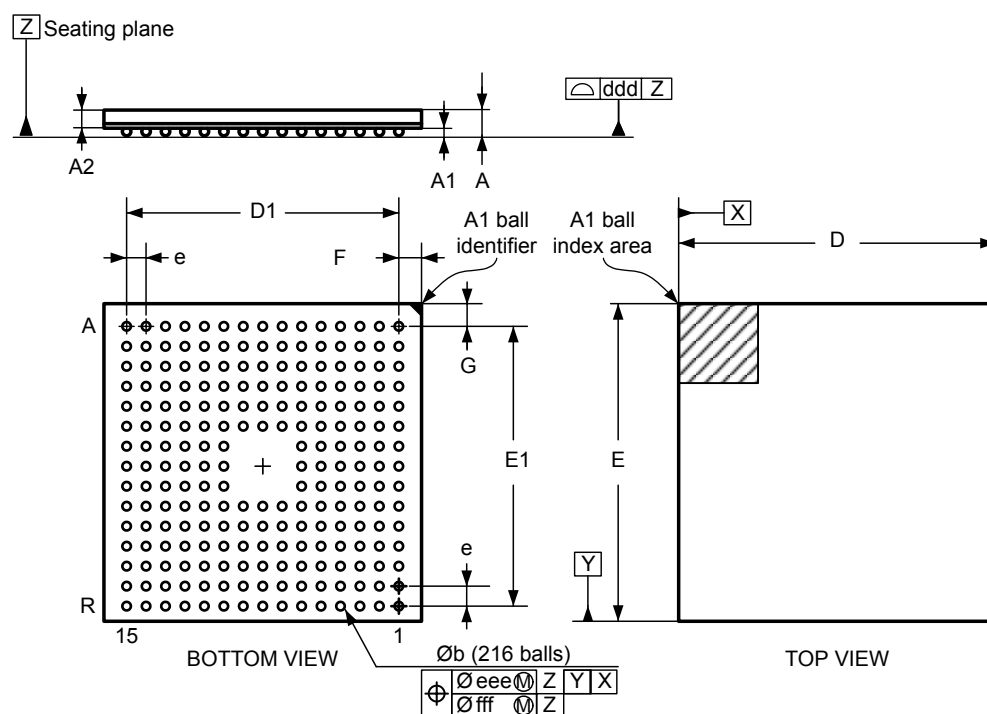
Figure 100. TFBGA216 - Outline
