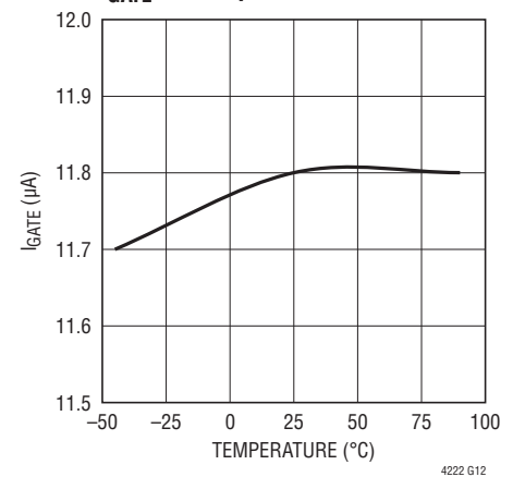
I_{\text{GATE}} vs Temperature
