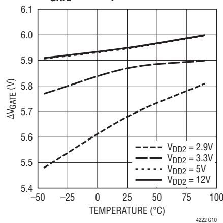
\Delta V_{\text{GATE}} vs Temperature
