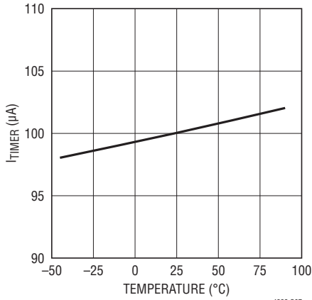
I_{\text{TIMER}} vs Temperature
