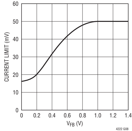
Current Limit vs V_{\text{FB}}
