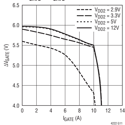
\Delta V_{\text{GATE}} vs I_{\text{GATE}}
