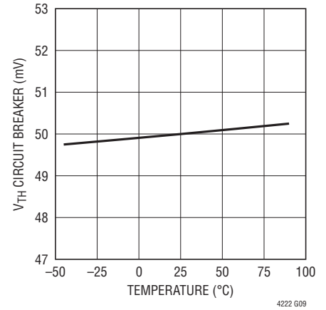
V_{\text{TH}} Circuit Breaker vs Temperature
