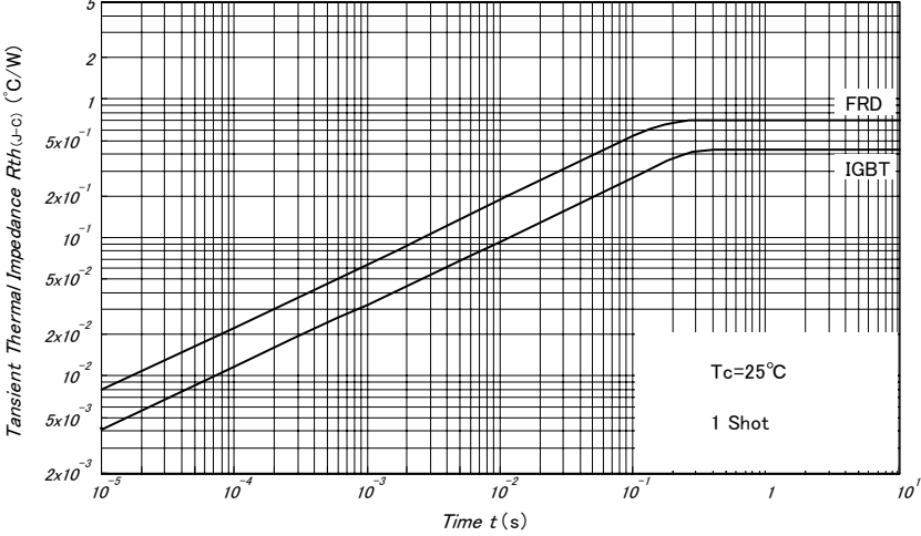
fig11-Tansient Thermal Impedance
