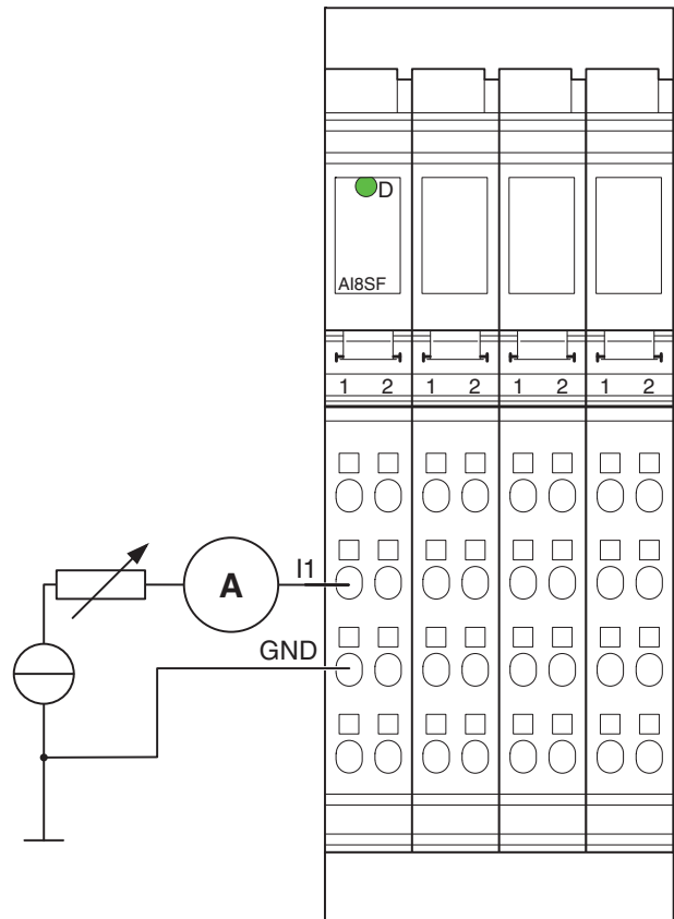
Figure 7 Measuring currents
