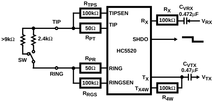
FIGURE 6. SWITCH HOOK DETECTION TEST CIRCUIT
