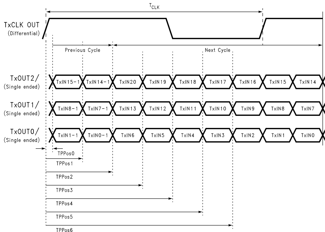
FIGURE 10. Transmitter LVDS Output Pulse Position Measurement
