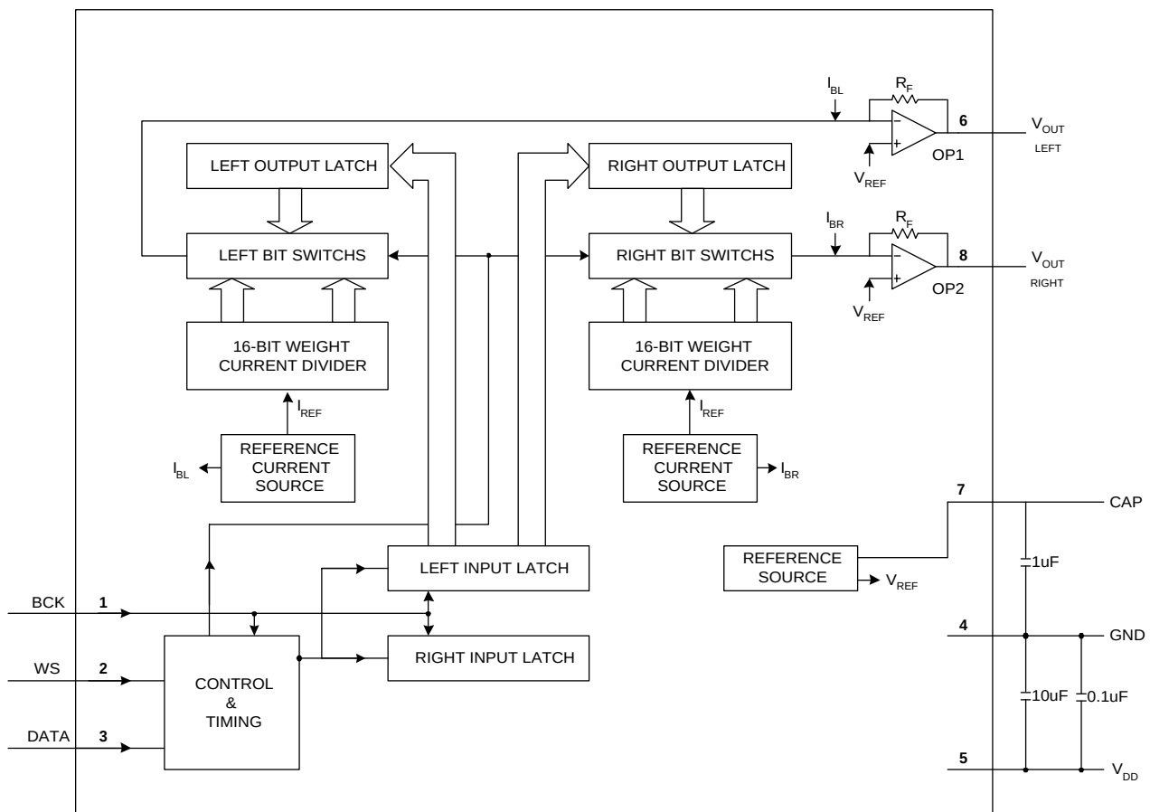
Fig.1 Block diagram.
