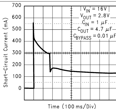
Figure 26. Short-Circuit Current
