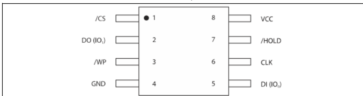
Figure 1a. W25X40CL Pin Assignments, 8-pin SOIC 208-mil, SOIC 150-mil and VSOP 150-mil (Package Code SS, SN & SV)
