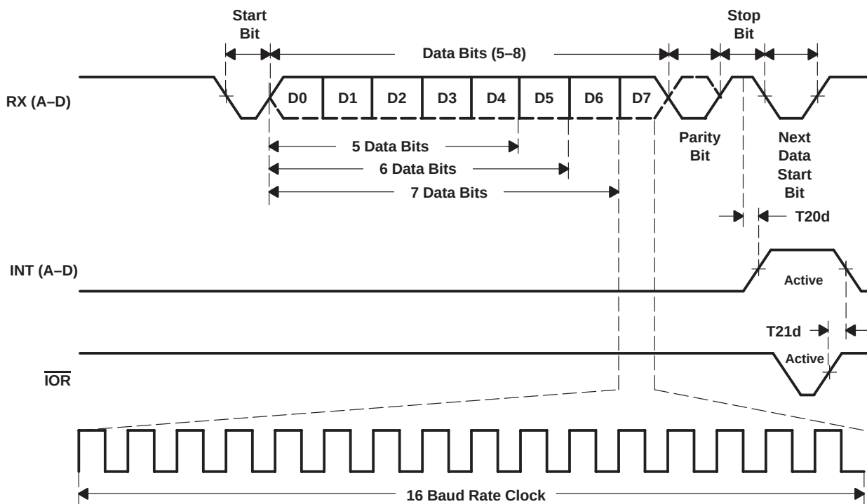
Figure 16. Receive Timing
