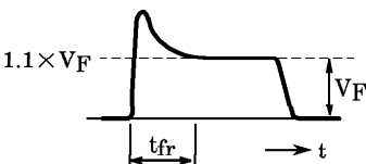
t_{fr} WAVEFORM
