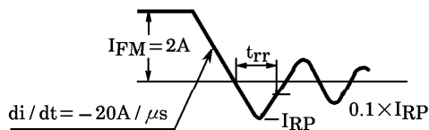
t_{rr} WAVEFORM
