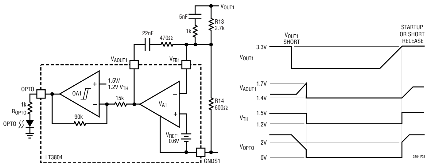
Figure 3. Optocoupler Driver
