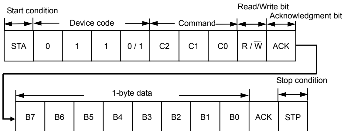
Figure 11 Data Communication
