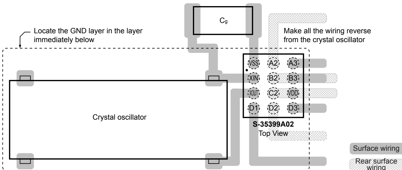
Figure 61 Connection Diagram 2
