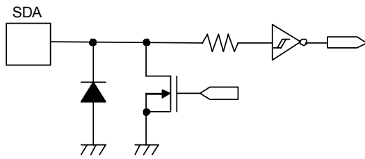
Figure 3 SDA Pin
