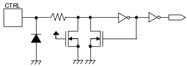
Figure 6 CTRL Pin
