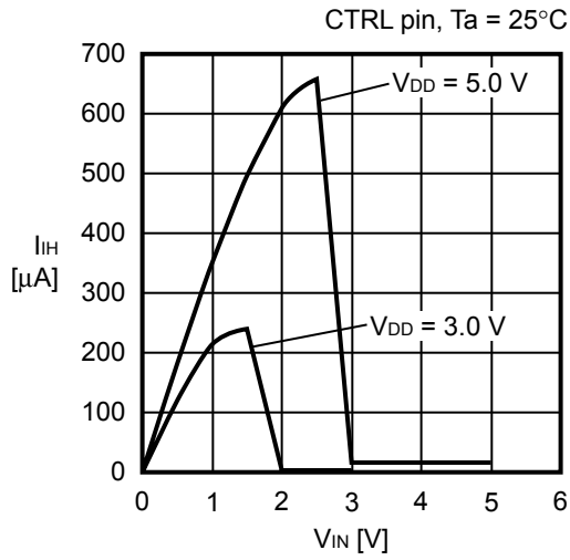
(13) Input current characteristics ( V_{IN} vs. I_{IH} )
