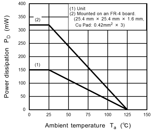
Fig. 7.4 P_D - T_a
