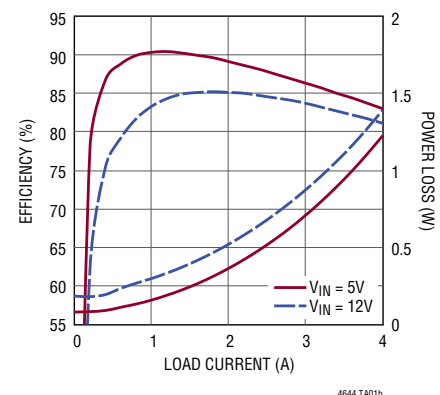
1.5V Output Efficiency and Power Loss (Each Channel)
