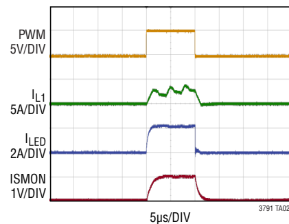
100Hz 1000:1 PWM Dimming ( V_{IN} = 24V )
