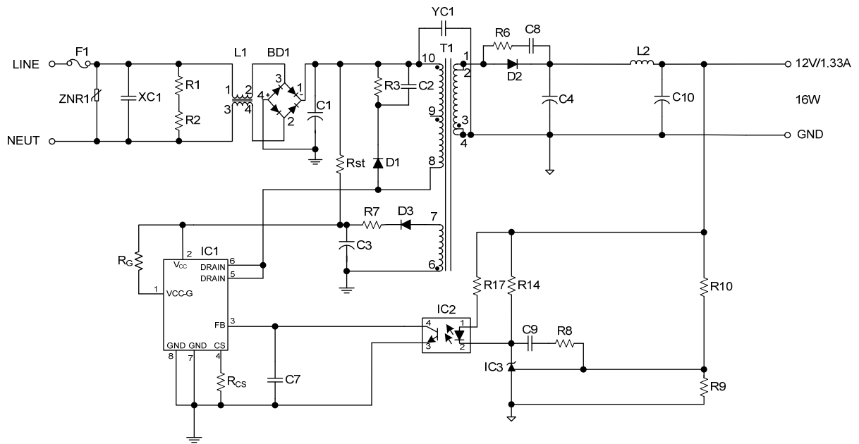
Fig.8 UTC US1652 Typical Application Circuit
