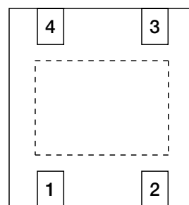
PLP-4B (TOP VIEW)
