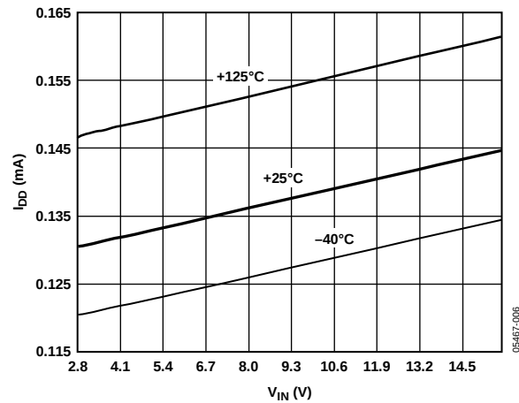
Figure 6. ADR361 Supply Current vs. Input Voltage
