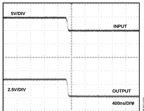
Figure 29. ADR361 Turn-Off Response Time at 5 V
