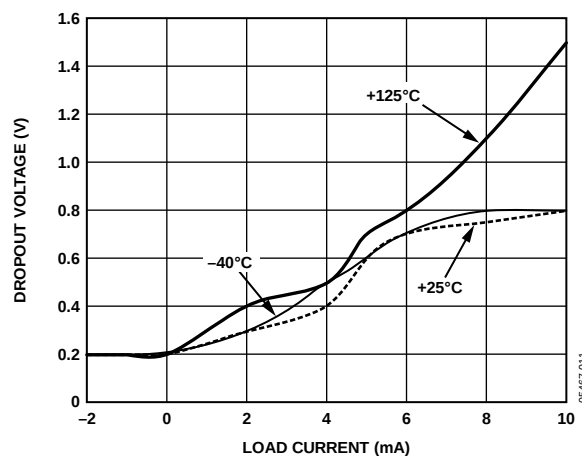
Figure 13. ADR361 Dropout Voltage vs. Load Current
