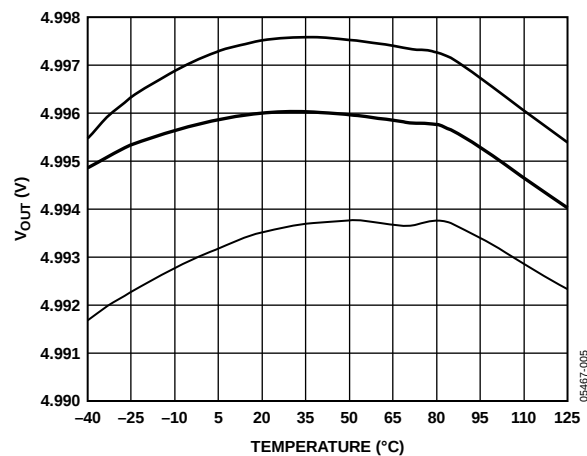
Figure 5. ADR365 Output Voltage vs. Temperature
