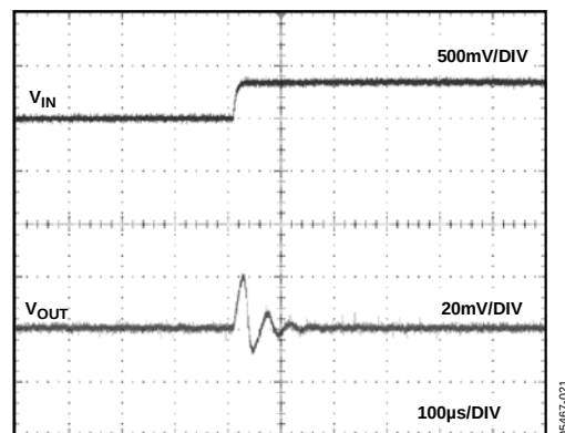
Figure 25. ADR361 Line Transient Response, 0.1 \mu F Input Capacitor
