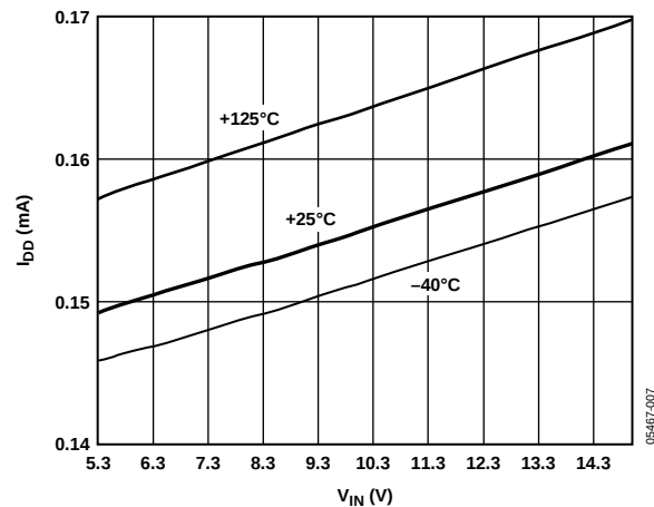
Figure 7. ADR365 Supply Current vs. Input Voltage
