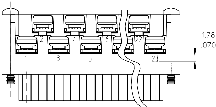
OPTIONAL 10A IMPRINTING (ODD CIRCUIT CONFIGURATION SHOWN)
