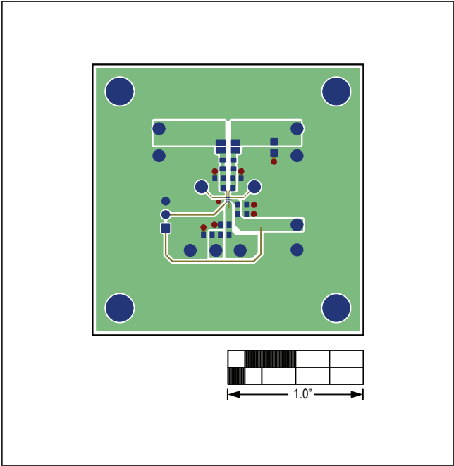
Figure 3. MAX44284 EV Kit PCB Layout—Component Side
