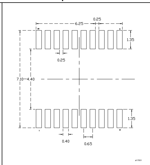
Figure 46. TSSOP20 recommended footprint (1)(2)
