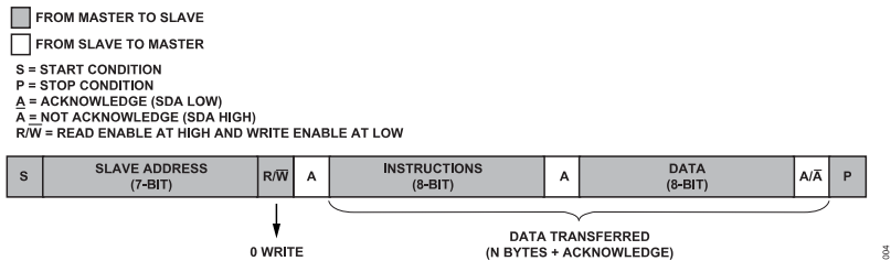
Figure 24. I 2 C—Master Writing Data to Slave
