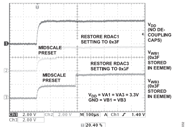
Figure 20. t_{\text{EEMEM\_RESTORE}} of RDAC1 and RDAC3
