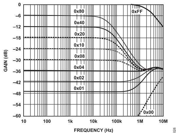
Figure 16. AD5252 Gain vs. Frequency vs. Code, R_{AB} = 100\text{ k}\Omega , T_A = 25^\circ\text{C}
