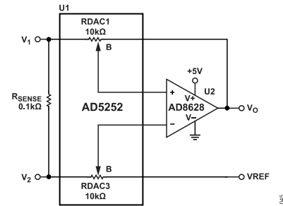
Figure 45. Current-Sensing Amplifier
