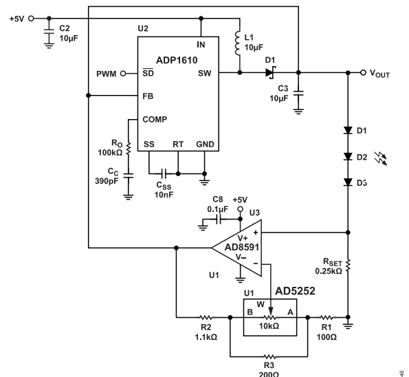
Figure 46. High Power, Adjustable LED Driver
