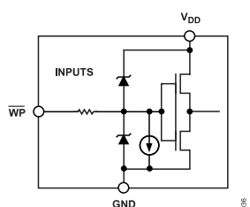
Figure 36. Equivalent \overline{WP} Digital Input
