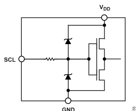
Figure 35. SCL Digital Input
