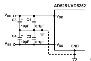
Figure 39. Power Supply-Bypassing Configuration
