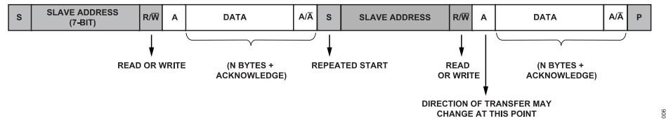
Figure 26. I 2 C—Combined Write/Read
