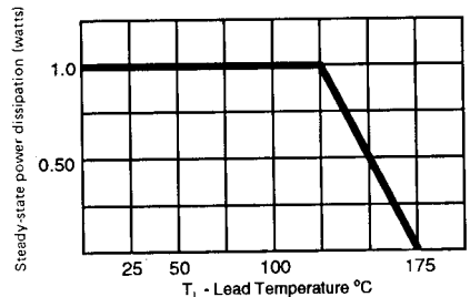
FIG. 4. Steady-state power derating curve
