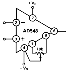
Figure 21. Offset Null Configuration
