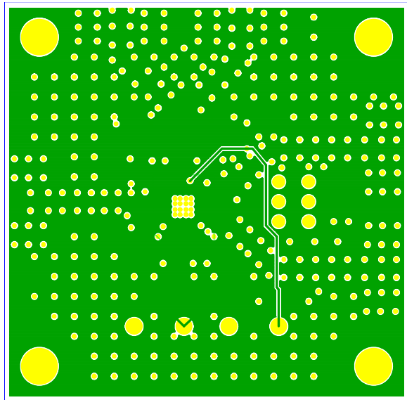
Figure 53. Evaluation Board Power Plane, Internal Layer 2
