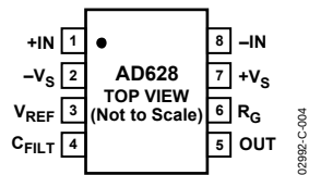
Figure 4. Pin Configuration
