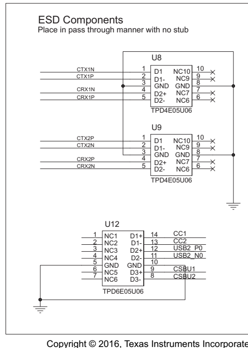
Figure 15. Schematic Implementations for DP Source/ USB Host (2 of 3)
