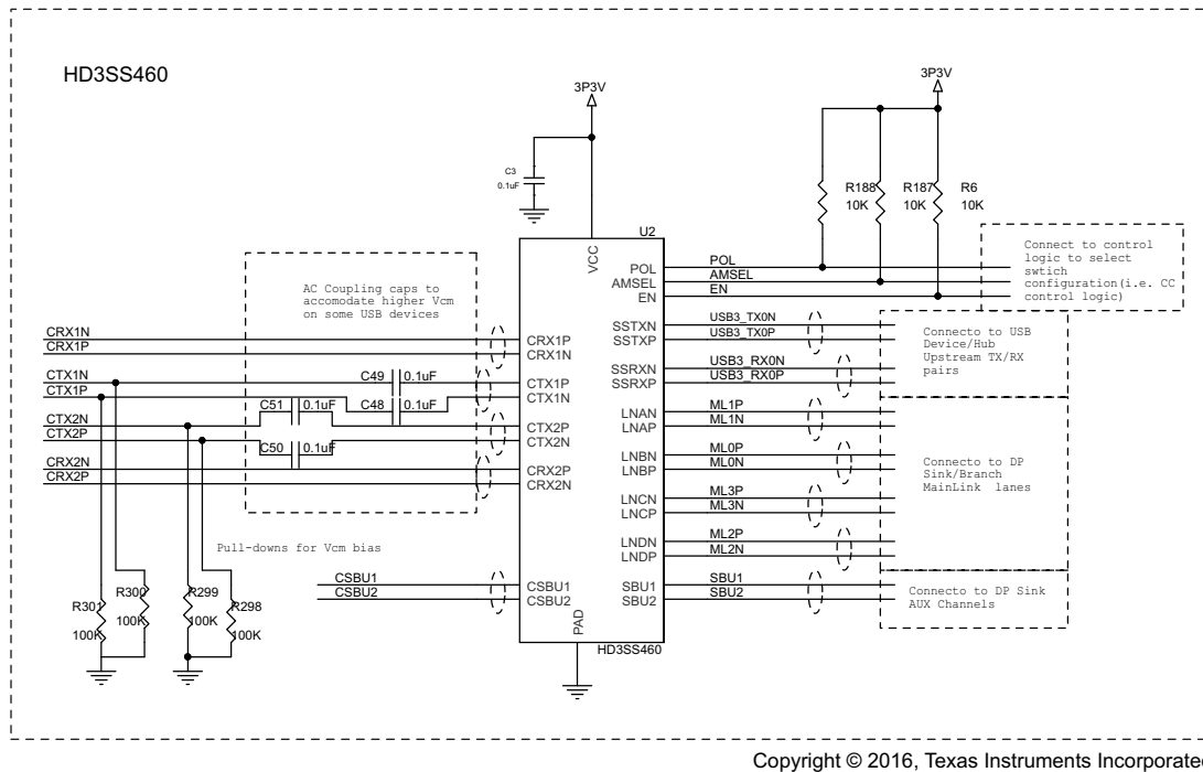
Figure 19. Schematic Implementations for DP Sink/ USB Device/HUB/Dock (3 of 3)
