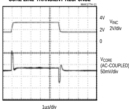
CORE LINE-TRANSIENT RESPONSE
