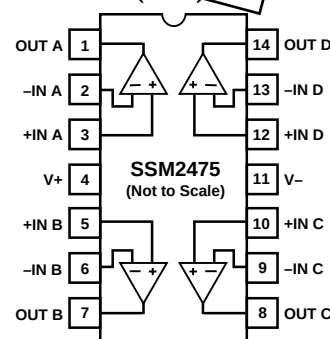
14-Lead Plastic DIP (N-14)
