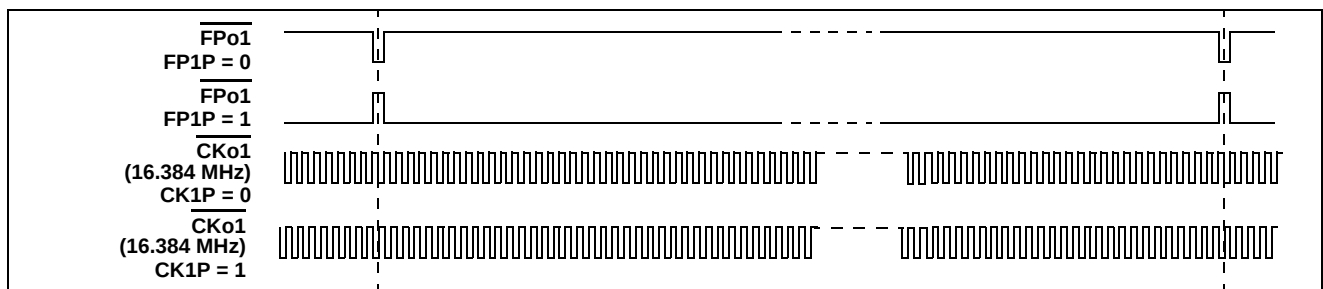
Figure 10 - FP01 and CK01 Output Timing when the CKFP1 Bit = 0
