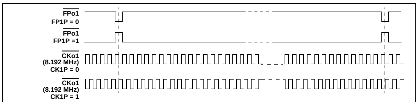
Figure 11 - FP01 and CK01 Output Timing when the CKFP1 Bit = 1
