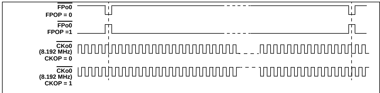
Figure 9 - FP00 and CK00 Output Timing when the CKFP0 Bit = 1
