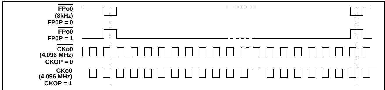
Figure 8 - FP00 and CK00 Output Timing when the CKFP0 Bit = 0
