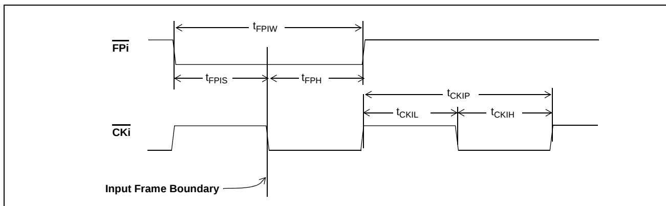
Figure 32 - Frame Pulse Input and Clock Input Timing Diagram
