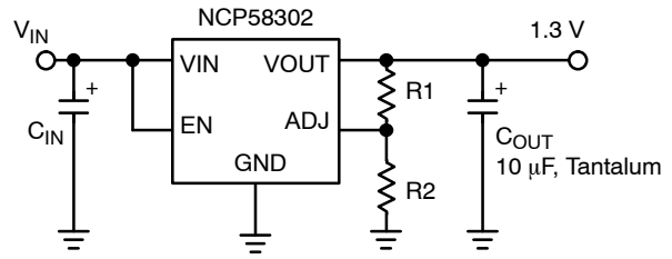
Figure 2. Adjustable Regulator
