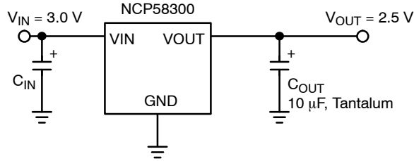
Figure 3. Fixed 2.5V Regulator in D 2 PAK-3 Package
