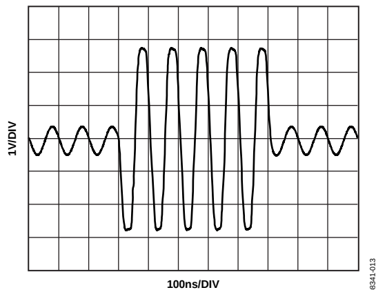
Figure 33. Overdrive Recovery, G = 24.08 dB
