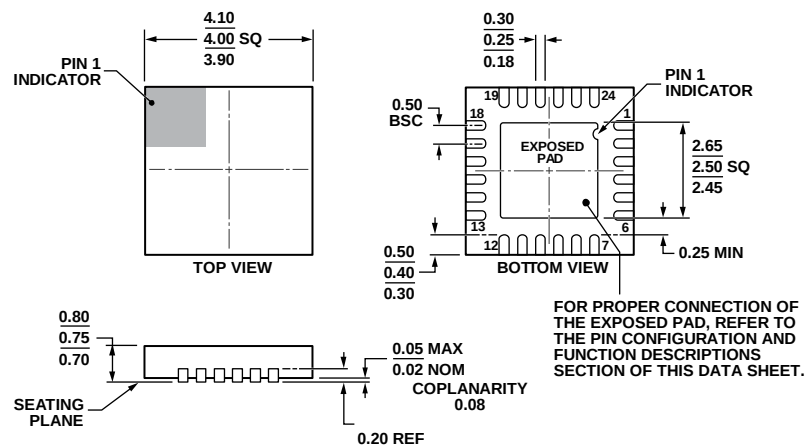
Figure 70. 24-Lead Lead Frame Chip Scale Package [LFSCP_WQ] 4 mm × 4 mm, Very Very Thin Quad (CP-24-7) Dimensions shown in millimeters
