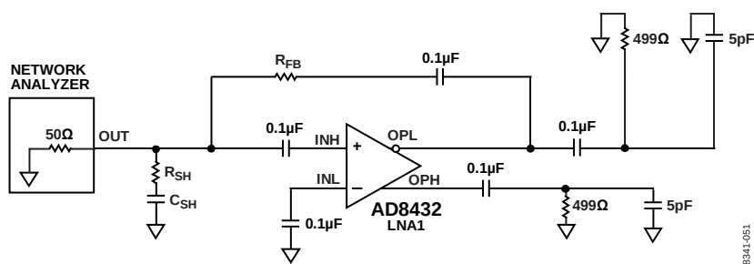
Figure 57. Input Impedance vs. Frequency Measurements
