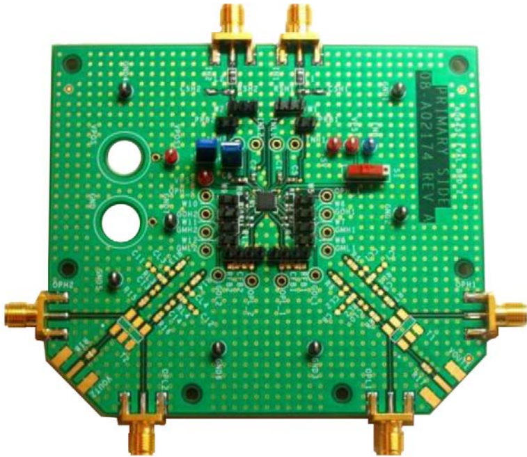
Figure 68. Evaluation Board
